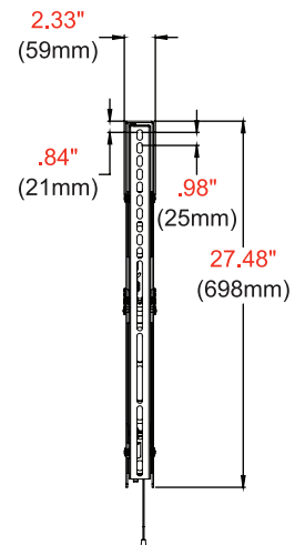
ADAPTER-DETAILS
